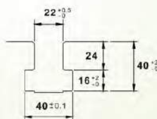
T型槽尺寸 T-slot size (LGN-25~110 tons)
