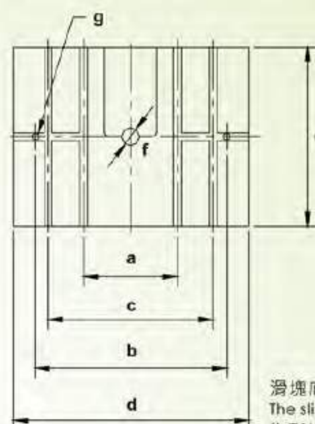
滑塊底面尺寸 The slider base size (LGN-25~110 tons)
