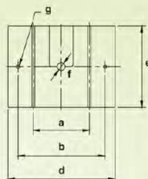
滑塊底面尺寸 The slider base size (LGN-25~110 tons)
