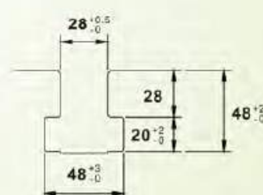
T型槽尺寸 T-slot size (LGN-160~260 tons)
